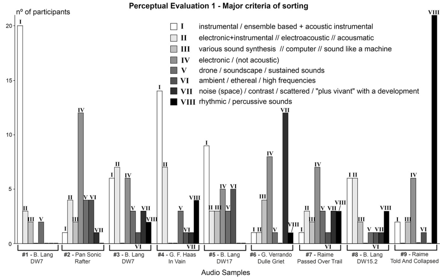
Figure 1. Major sorting criteria (I–VIII) for audio samples (1–9) used in the Perceptual Evaluation #1.
