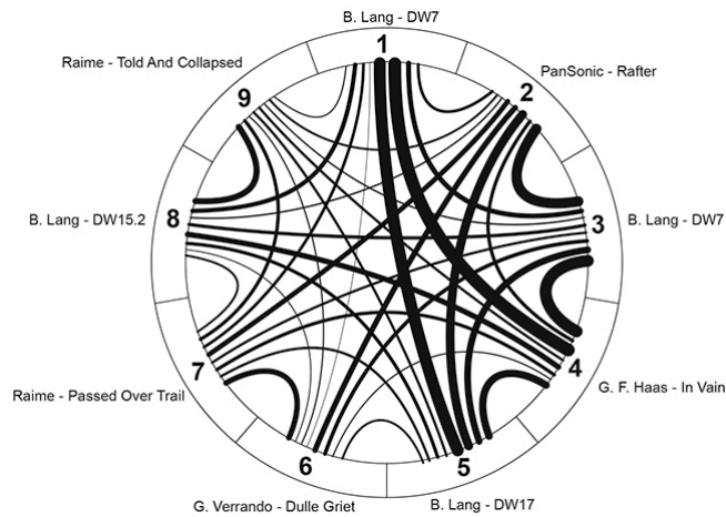
Figure 2. Sorting for groups of two samples: the thicker is the connecting line the higher number of participants associates the respective pieces.
